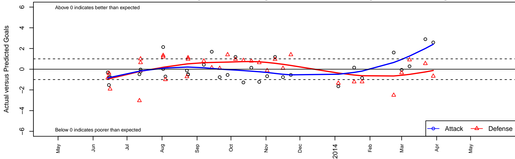
Seattle United NE White G99 Dots are actual minus expected GF (blue circles) and GA (red triangles). Blue line is smoothed change in attack strength. Red is smoothed change in defense strength.
